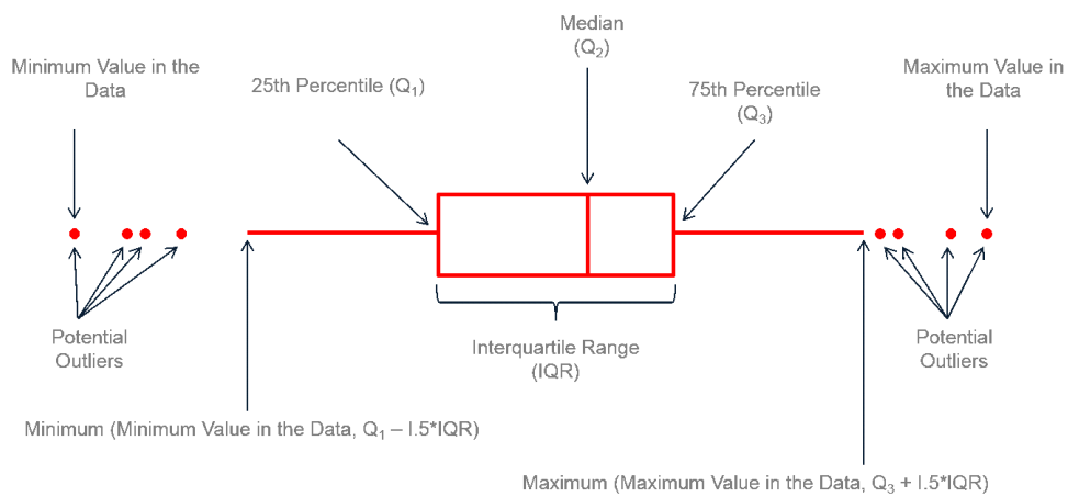
Abbildung 6.17: Boxplot Anatomie. Quelle: https://www.leansigmacorporation.com/box-plot-with-minitab/
